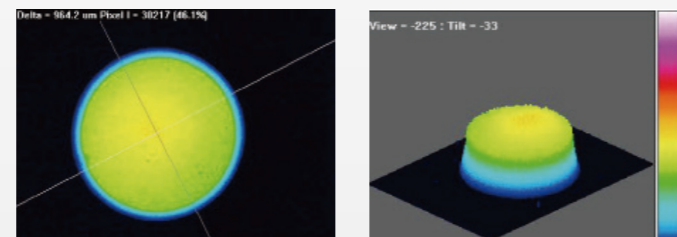
Photograph by Beam Profiler (gentec, "Beamage")
